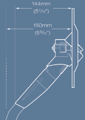
Angled Housing
