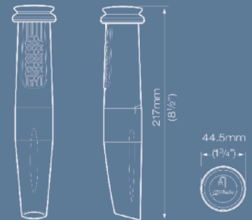
Handset
